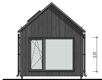
F2 ELEVATION 1:80
