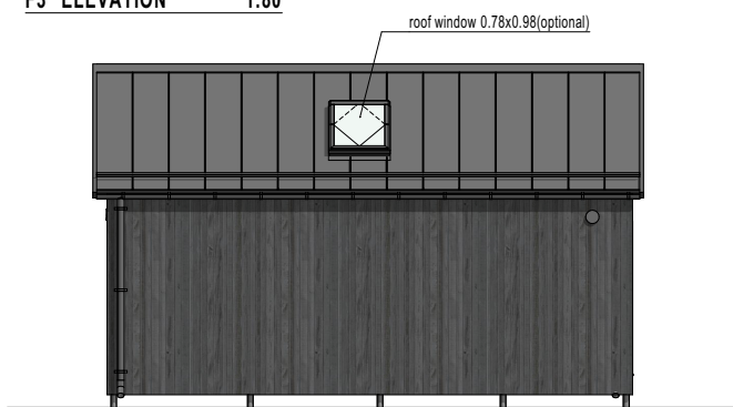
F3 ELEVATION 1:80
