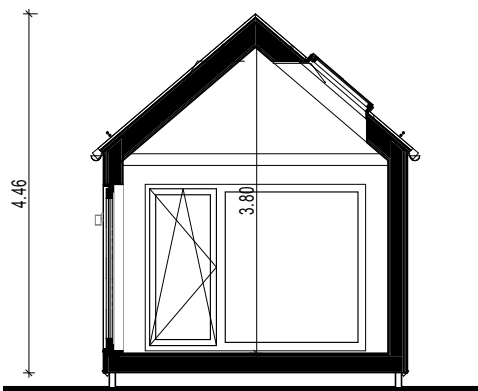
A SECTION 1:80
