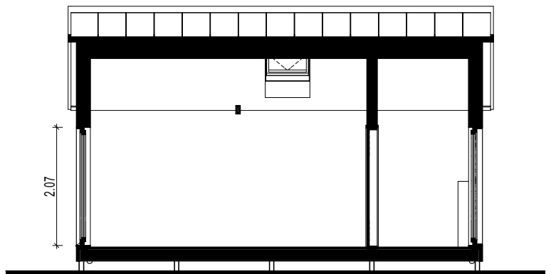
B SECTION 1:80
