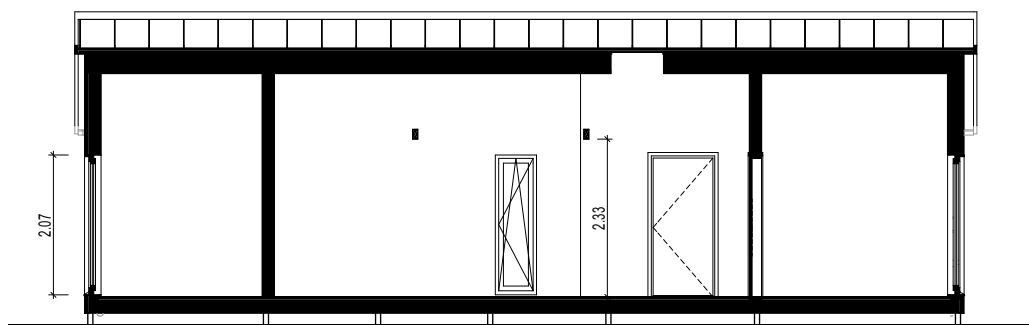
C SECTION 1:80
