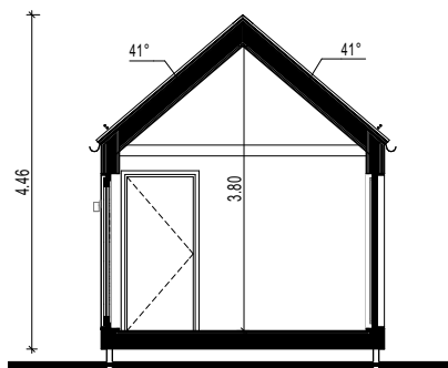
C SECTION 1:80
