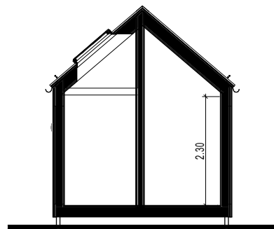
B SECTION 1:80
