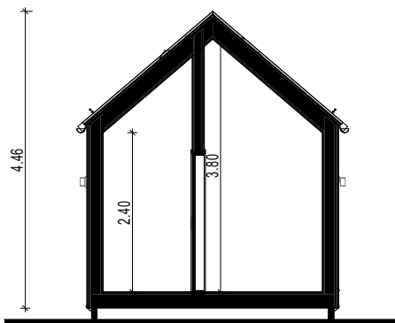
A SECTION 1:80
