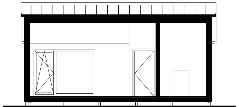
B SECTION 1:80
